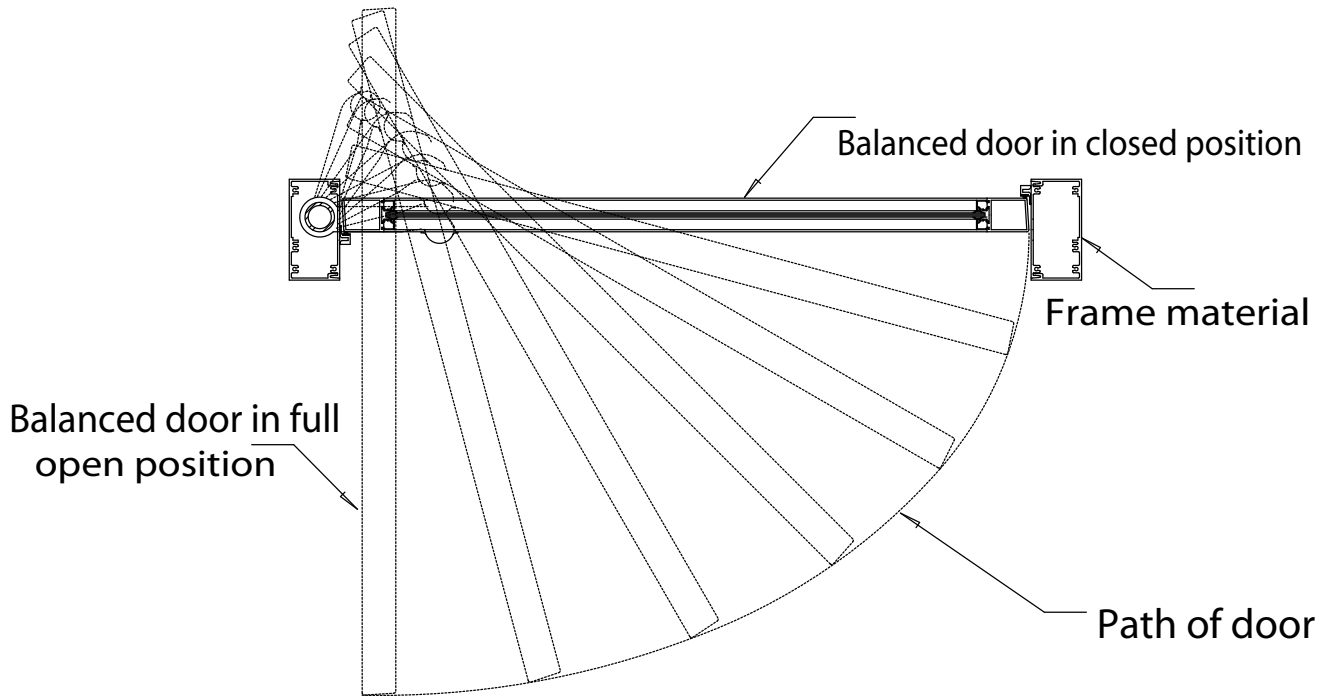
Balanced door plan drawing showing opening path of door
