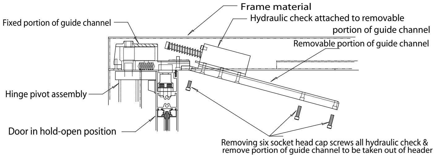
Partial elevation detail "B" showing check and removable portion of guide channel being removed from header while door is in hold-open position
